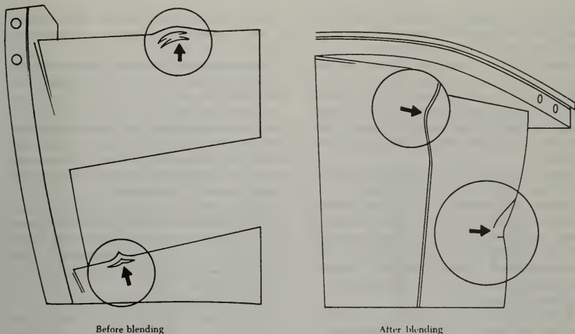
FIGURE 10-57. Guide vane trailing edge damage.
